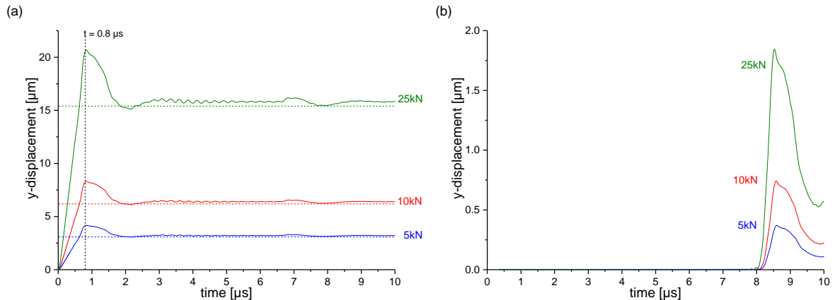
Fig. 5. Evaluation of source displacement (a) and surface displacement at (x,y) = (0,50) mm (b) as function of external load.
